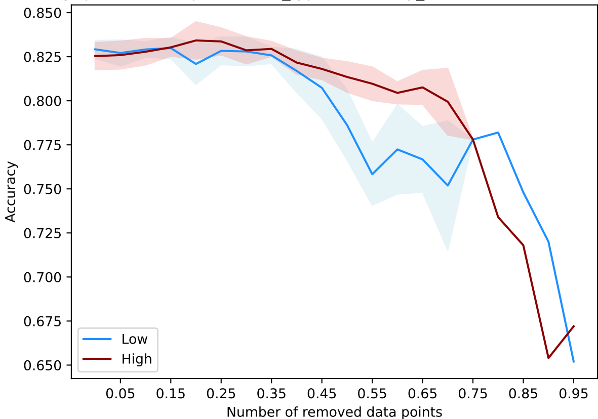
PruningOptimization(optimization_type=size, only_size=50) - imdb-embed
